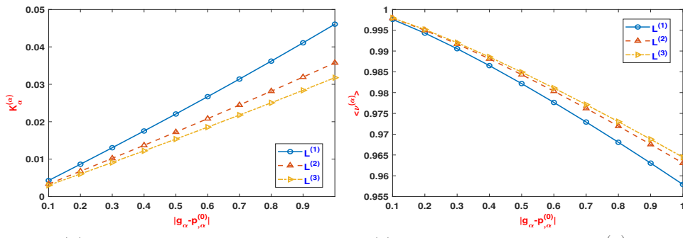
Figure 2. The relationships between the permeability tensor K_\alpha^\alpha and effective viscosity \mu^{(\alpha)} of a Carreau-Yasuda fluid.
